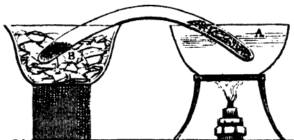
Fig. 142. The Liquefaction of Ammoniacal Gas. A. Extremity of the bent-glass tube containing the chloride of silver saturated with dry ammoniacal gas, and placed in a copper pan containing water, and gently heated by the spirit-lamp below. B. The other end of the tube surrounded with ice, where the liquefaction of the gas takes place by its own pressure and the cold.
